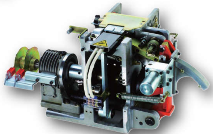
Low maintenance strap feeding and tensioning module
